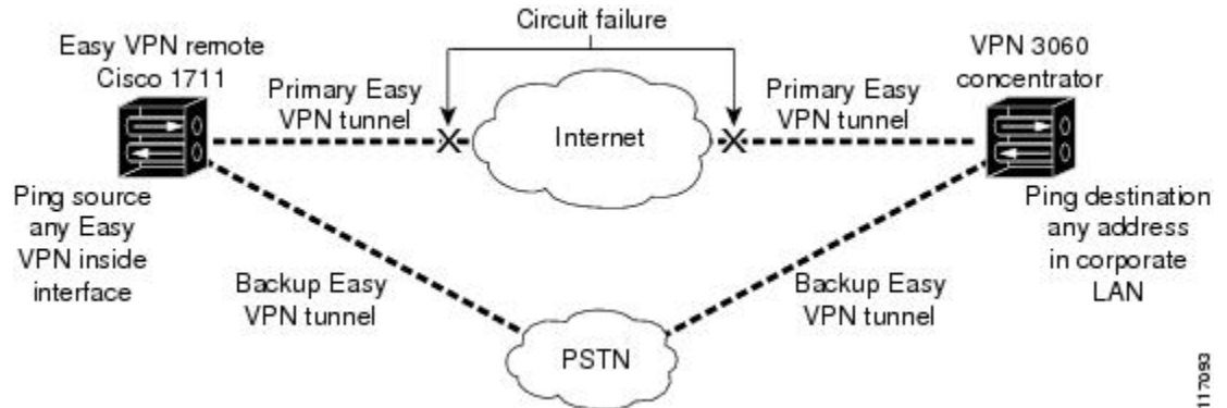
Figure 10: Dial Backup for Easy VPN Scenario
