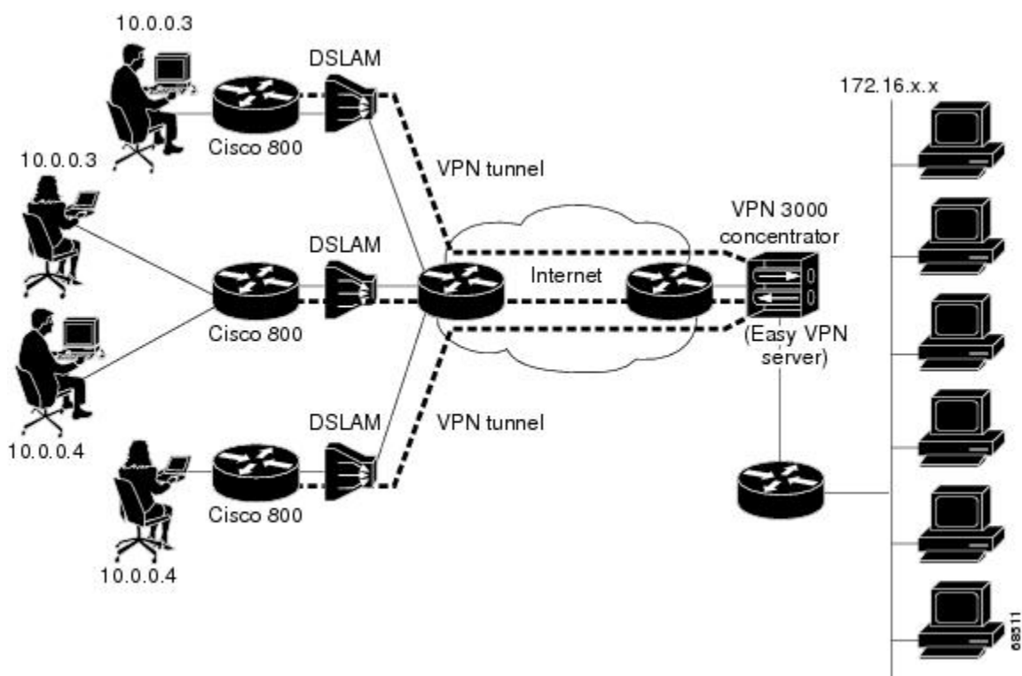
Figure 2: Cisco Easy VPN Remote Connection (Using a VPN Concentrator)
